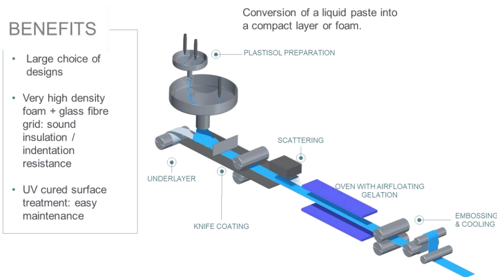
Figure 8: Coating process
