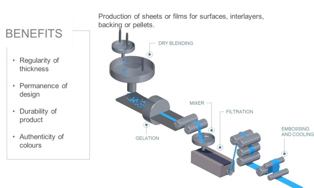
Figure 9: Calendering process
